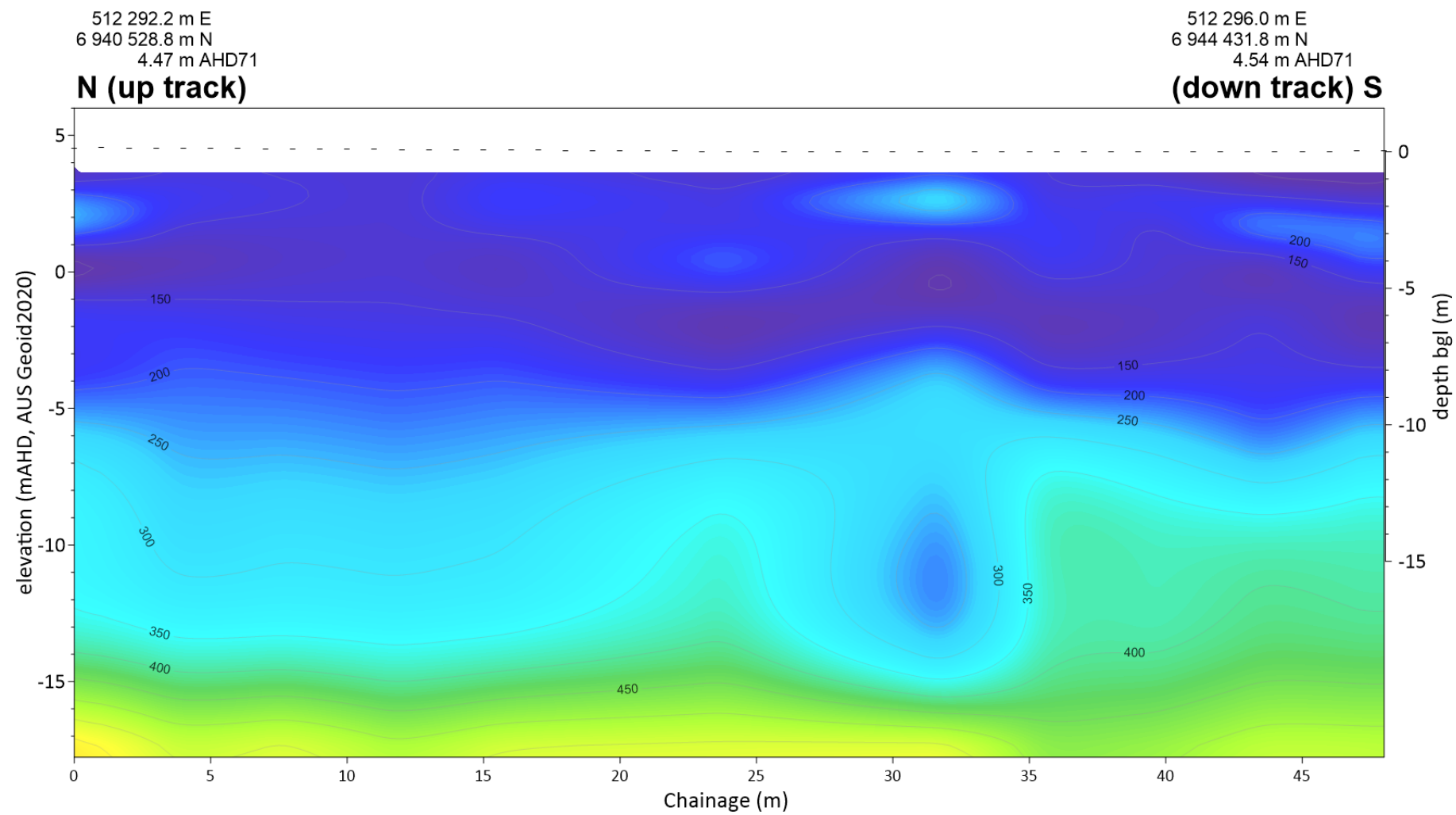
Seismic Line MASW AU-GP 144
